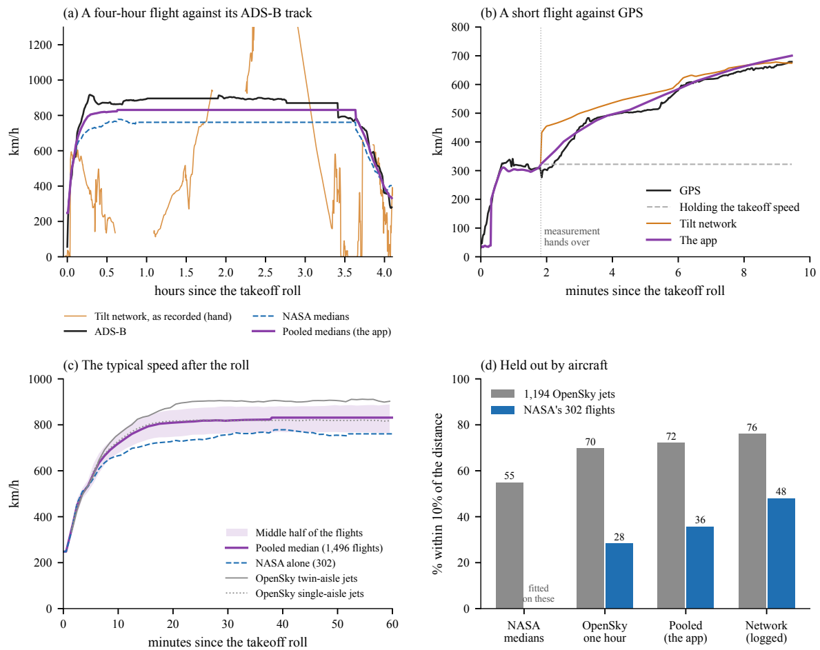
Figure 5. Speed in the air. (a) The four-hour flight against its ADS-B track: the typical flight of NASA’s jet, the pooled flights the app uses, and the tilt network the app used before, as the phone in a hand recorded it. (b) The short flight against GPS: the takeoff is measured until the dotted line, then the typical flight carries what it measured; holding the measured speed misses the climb. (c) The typical speed after the roll: the pooled median and the middle half of the flights, NASA’s jet alone, and OpenSky’s twin- and single-aisle jets. (d) Flights within 10% of the distance from the roll to landing, each measured without its own aircraft.
