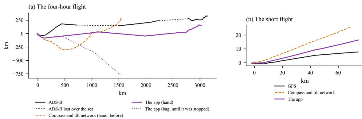
Figure 7. The flights drawn with no GPS after the first point. (a) The four-hour flight: its ADS-B track (dashed where the receivers lost it over the sea), the app with the phone in a hand and in a bag (until it was stopped), and the compass and tilt network the app used before. (b) The short flight against GPS. Like the example routes in Figures 2 and 4 they are turned by an arbitrary angle, on a plain km grid, so as not to show where they were recorded.
