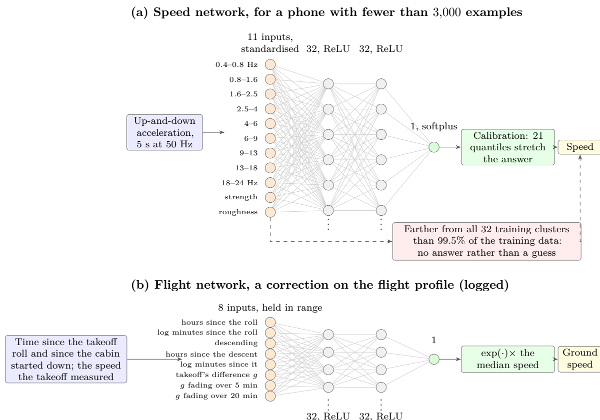
Figure 8. The two built-in networks, drawn layer by layer; each hidden layer has 32 units, of which only some are drawn. (a) The speed network: the fingerprint's eleven numbers go through two layers of 32 and one output, which a calibration then stretches; a fingerprint unlike any it was trained on gets no answer. (b) The flight network: the time since the takeoff roll and since the cabin started down, and the difference the takeoff measured, go through the same two layers; the output scales the typical speed.
