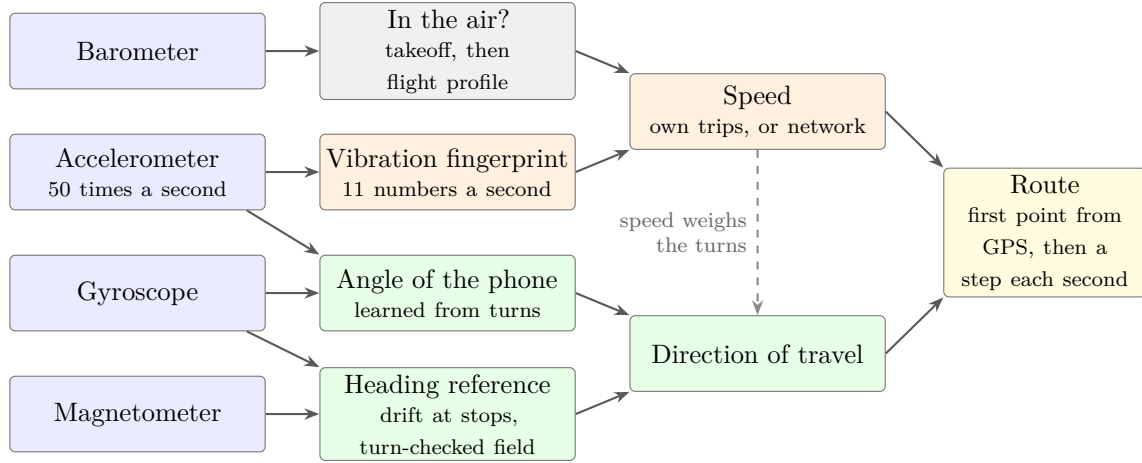
Figure 1. The system. Speed comes from the accelerometer’s vibration, or in the air from integrating the takeoff and then from the typical speed of real airline flights; direction combines the angle of the phone, learned from the gyroscope’s turns and the push felt in them, with a heading reference. GPS gives the first point and nothing else.
